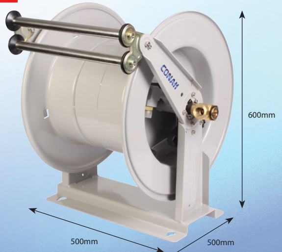
Spring Rewind Without Hose, 3/4"
