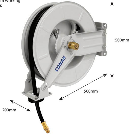
Rubber Air Hose, Spring Rewind, 1/2"
