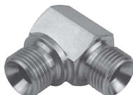
BSPP Male x BSPP Male 90° Compact Elbow for Bonded Seal 60° Cone
