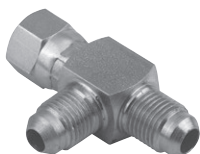
JIC Male x JIC Swivel Female x JIC Male Branch Tee 37° Cone
