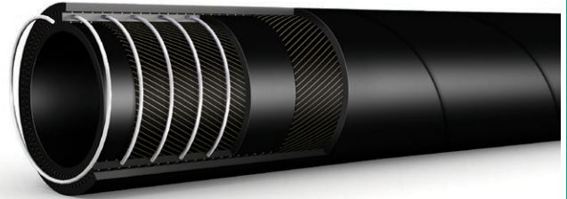
RBR-12 19mm (0.75 in) DN19 21 bar (305 psi) SAE100R4
