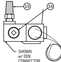
VIEW C – SOLENOID VALVE
