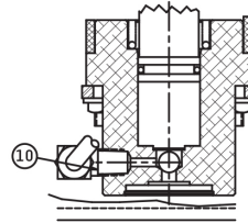
VIEW A – SLR & PROGRESSIVE MODELS
