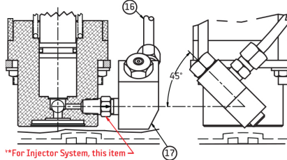
VIEW B - PDI MODELS & INJ MODELS
